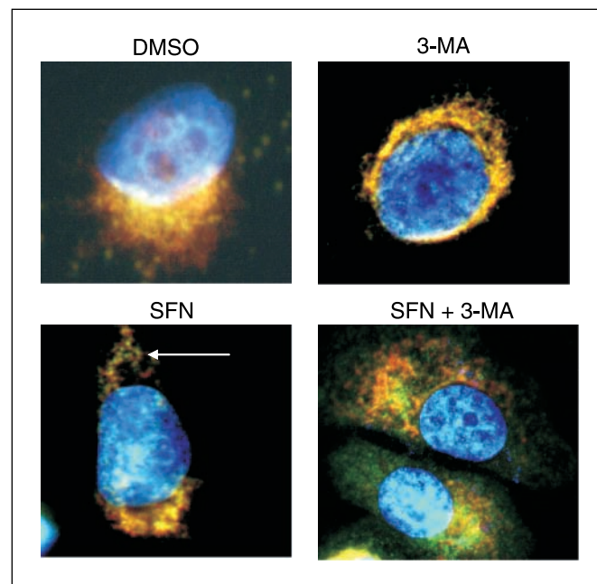
Figure 5. Immunocytochemistry for cytochrome c localization in PC-3 cells treated for 9 hours with DMSO (control) or 40 \mu\text{mol/L} sulforaphane in the presence or absence of 10 mmol/L 3-MA. Staining for cytochrome c (green fluorescence), MitoTracker Red (mitochondria; red fluorescence), and DAPI (nuclei; blue fluorescence). In cells treated with DMSO or 3-MA alone, cytochrome c was primarily localized in mitochondria as revealed by a yellow-orange staining due to merging of red (mitochondria) and green fluorescence (cytochrome c ). Sulforaphane treatment alone caused translocation of cytochrome c from mitochondria to the cytosol evidenced by appearance of green fluorescence in the cytoplasm (arrow). Cytosolic cytochrome c (green fluorescence) was much more pronounced in PC-3 cells treated with sulforaphane plus 3-MA. Similar results were observed in replicate experiments.
