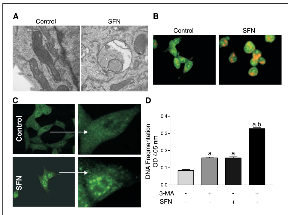
Figure 6. A, representative electron micrographs depicting ultrastructures of LNCaP cells treated for 6 hours with DMSO or 40 \mu M/L sulforaphane. Note the healthy-looking mitochondria in control cells and membranous vacuoles in sulforaphane-treated LNCaP cells. Magnification, \times 50,000 . B, acridine orange staining in LNCaP cells treated for 6 hours with either DMSO (control) or 40 \mu M/L sulforaphane. Similar results were observed in two independent experiments. C, immunocytochemistry for LC3 localization in LNCaP cells treated for 6 hours with DMSO or 40 \mu M/L sulforaphane. Right, enlarged images of the cells marked by arrows. D, cytoplasmic histone-associated DNA fragmentation in LNCaP cells treated with DMSO (control) or 10 \mu M/L sulforaphane in the presence or absence of 10 mmol/L 3-MA. Columns, mean ( n = 3 ); bars, SE. a, P < 0.05 , significantly different compared with DMSO-treated control; b, P < 0.05 , significantly different compared with sulforaphane-alone treatment group by one-way ANOVA followed by Bonferroni's multiple comparison test. Similar results were observed in replicate experiments.
